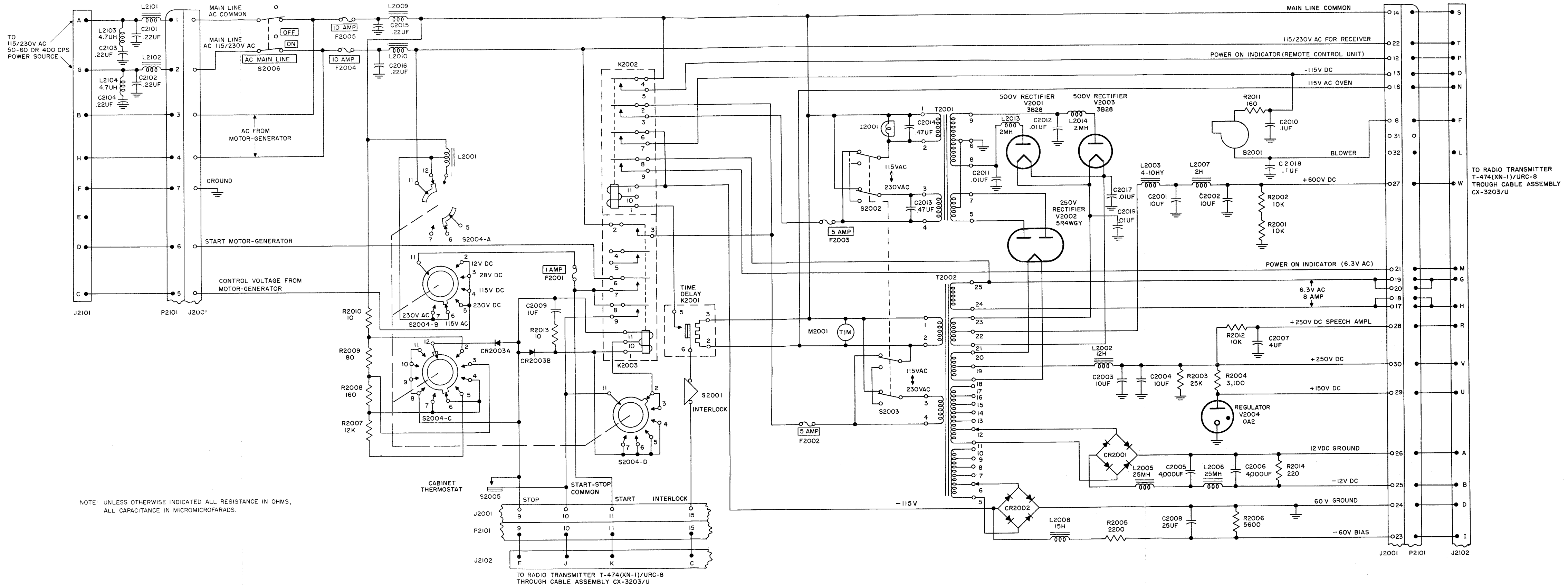
Figure 5-7. Power Supply PP-1190(XN-1)/URC-8, Schematic Diagram
