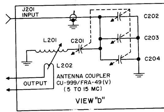
Figure 6-18. Antenna Coupler Group AN/FRA-49(V), Schematic Diagram
