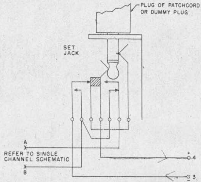
Figure 2-2. Dummy Plug or Patchcord in Set Jack
