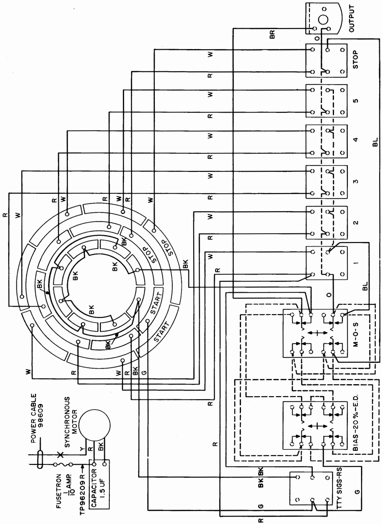
Fig. 3 - 100A Teletypewriter Test Distributor - Wiring Diagram
