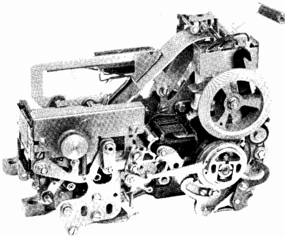
Figure 6 - Typical Reperforator Unit
