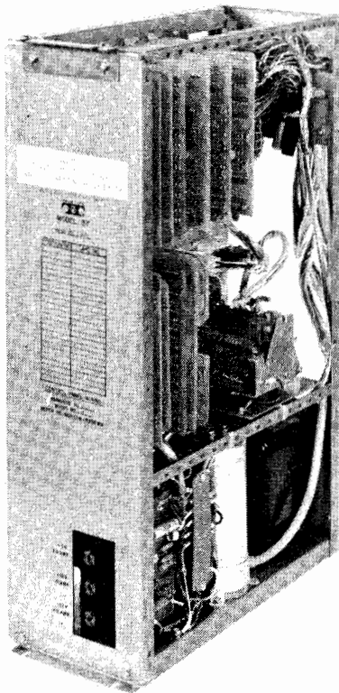
Figure 5 - Typical Electrical Service Unit
