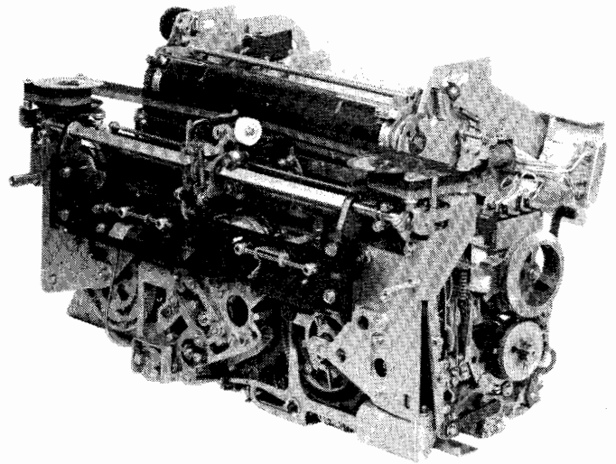
Figure 2 - Typical Typing Unit
