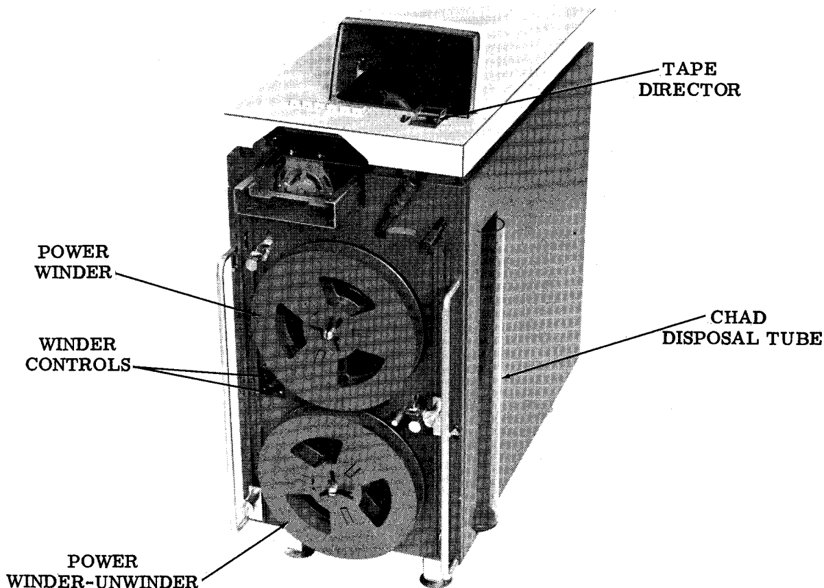
Figure 9 - Tape Handling Accessories
