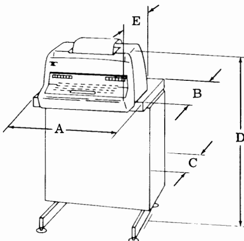
SINGLE-COMPARTMENT TABLE (Standard Depth)
