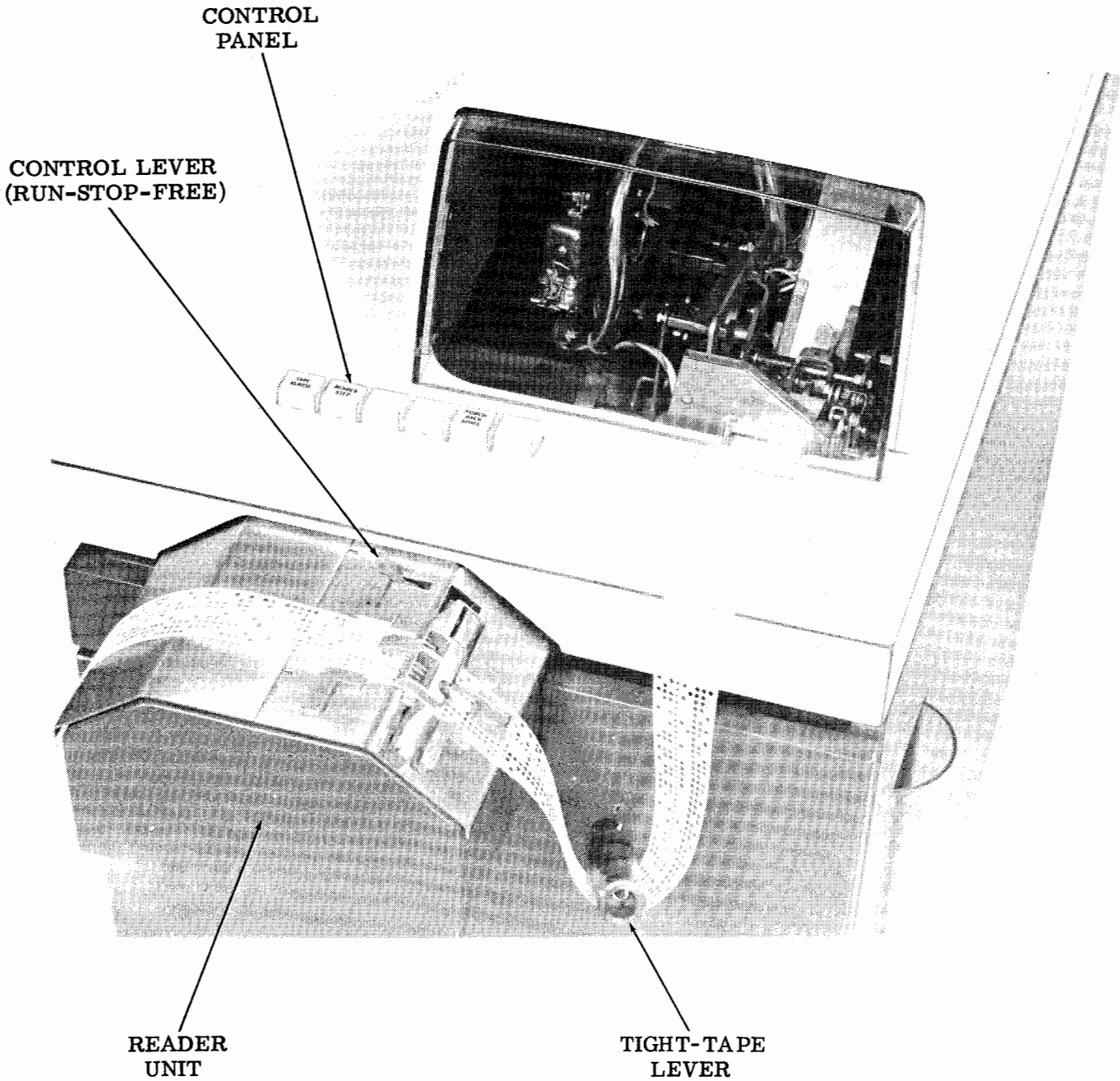
Figure 8 - RT Module Controls
