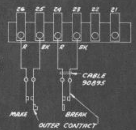
A BREAK-LOCK CONTACTS ONLY
