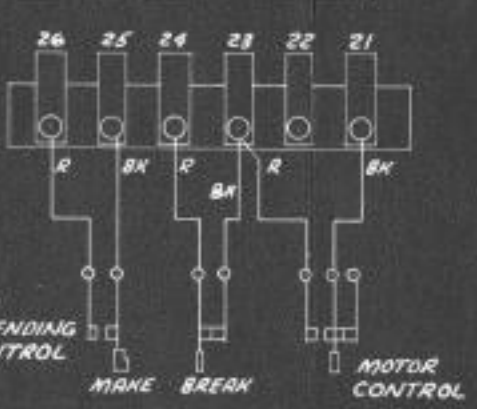
D BREAK-LOCK AND MOTOR CONTROL
