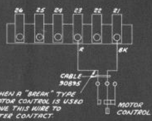
B MOTOR CONTROL ONLY
