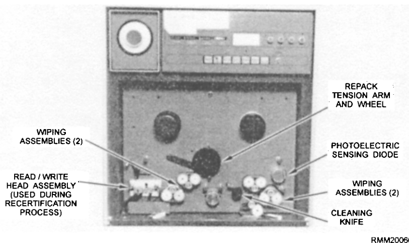
Figure 2-12.—Tape cleaner/certifier.
