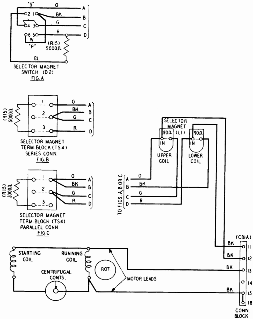
Figure 1 – 14AG, 14AH, 14AP Typing Units, and 14M, 14P, 14S, 14T, 14AG, 14AH, 14AJ, 14AK, 14AK-1, and 14AL Typing Reperforator Units (Synchronous Motor)
