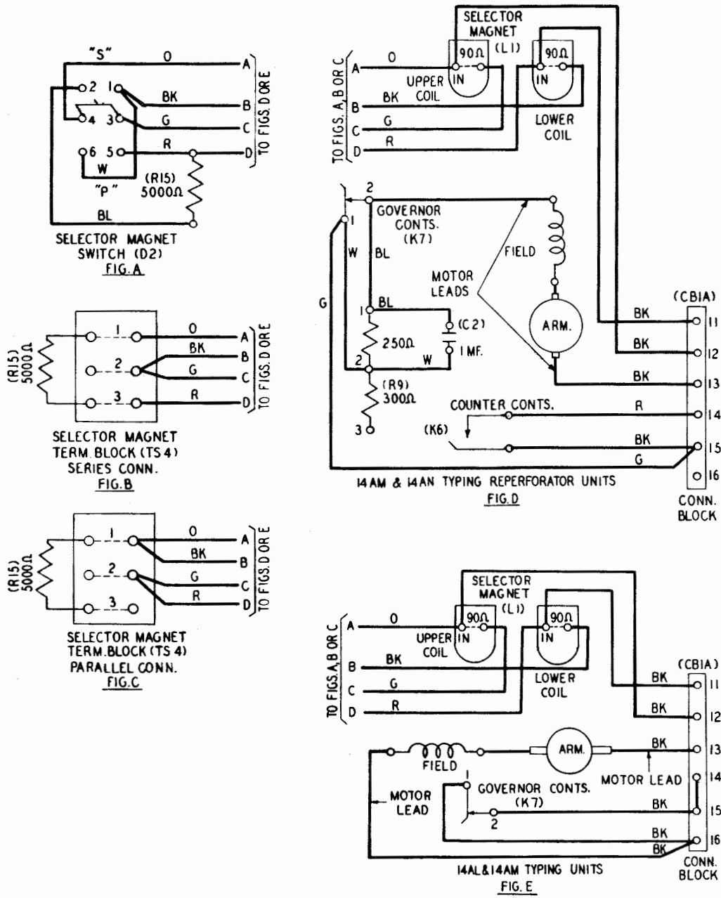
Figure 3 — 14AM, 14AN Typing Reperforator Units, and 14AL, 14AM Typing Units (AC Series Motor)
