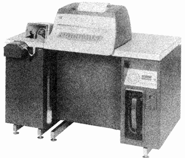
Figure 1 - 37 ASR Teletypewriter Set
