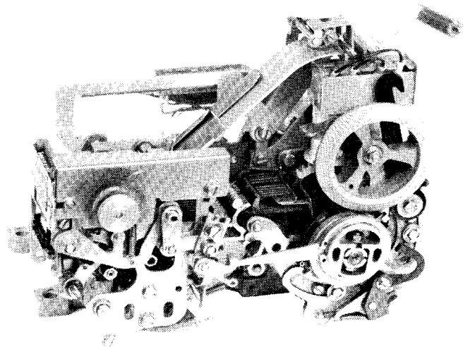
Figure 11 - Reperforator Unit
