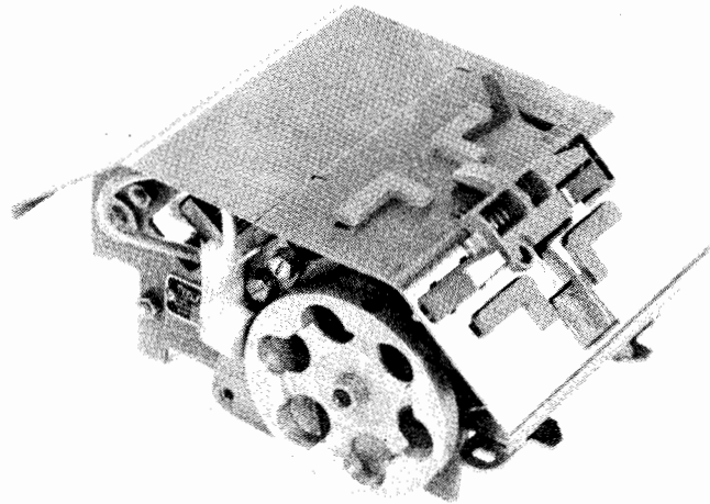
Figure 12 - Reader Unit
