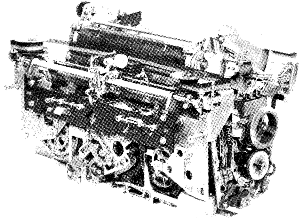
Figure 4 - Typing Unit
