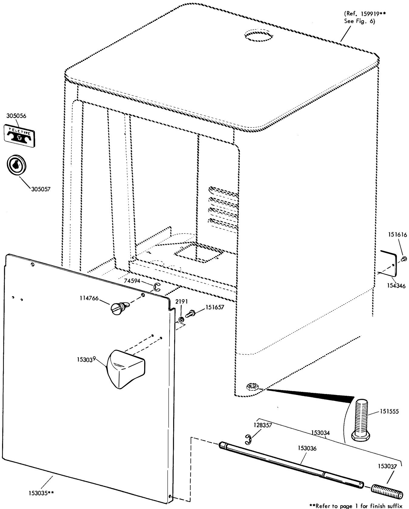
FIGURE 5. TABLE (w/Full Door)
