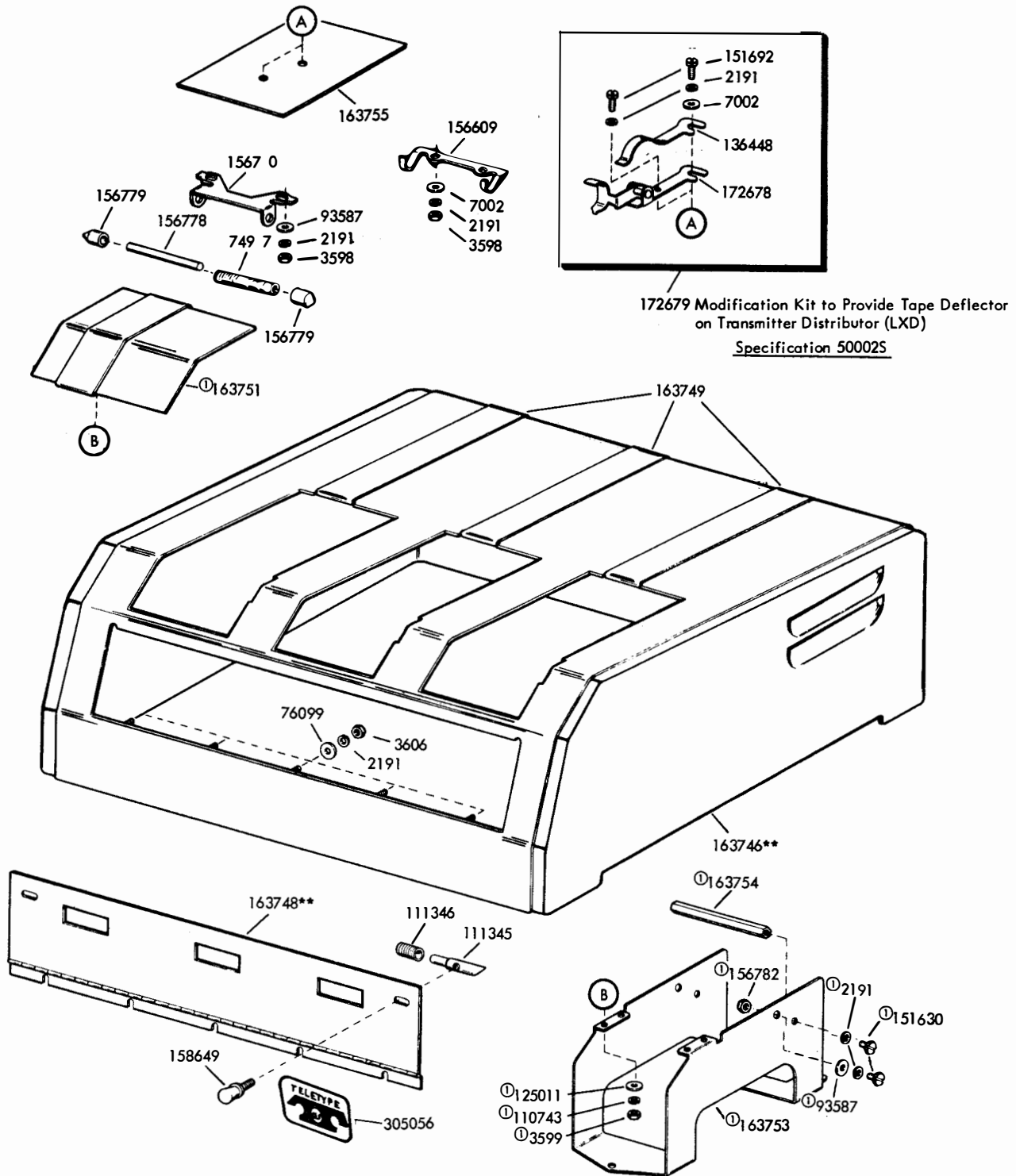
①163752 Modification Kit to Provide a Dummy Unit for the Multiple Transmitter Distributor Base. Specification 59815
