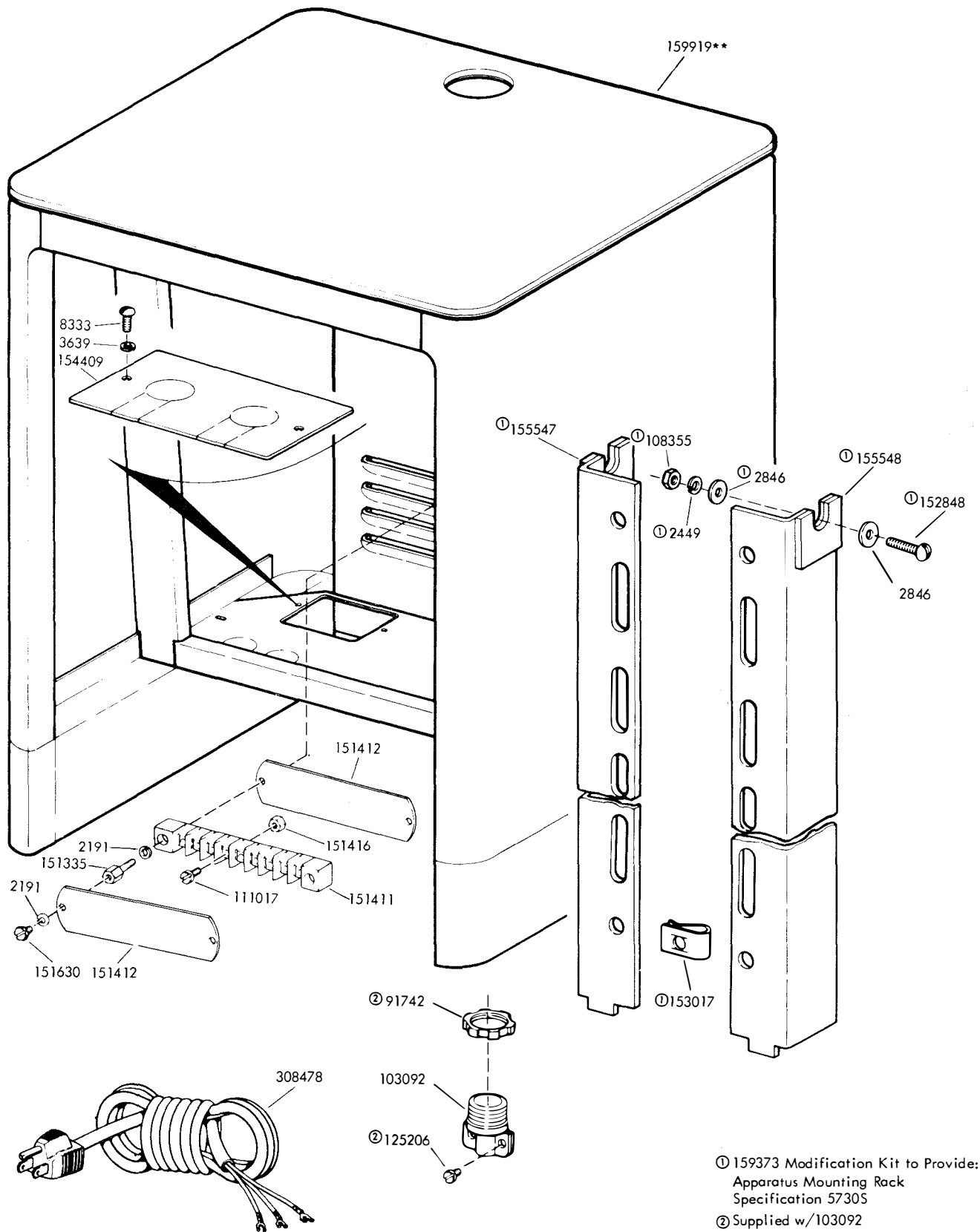
FIGURE 6. TABLE (w/Full Door - Continued)
