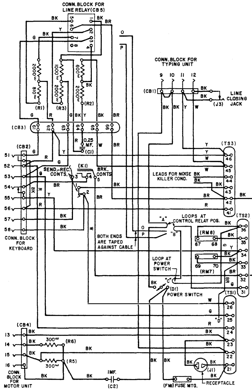
Figure 1- 15A Teletypewriter Base
