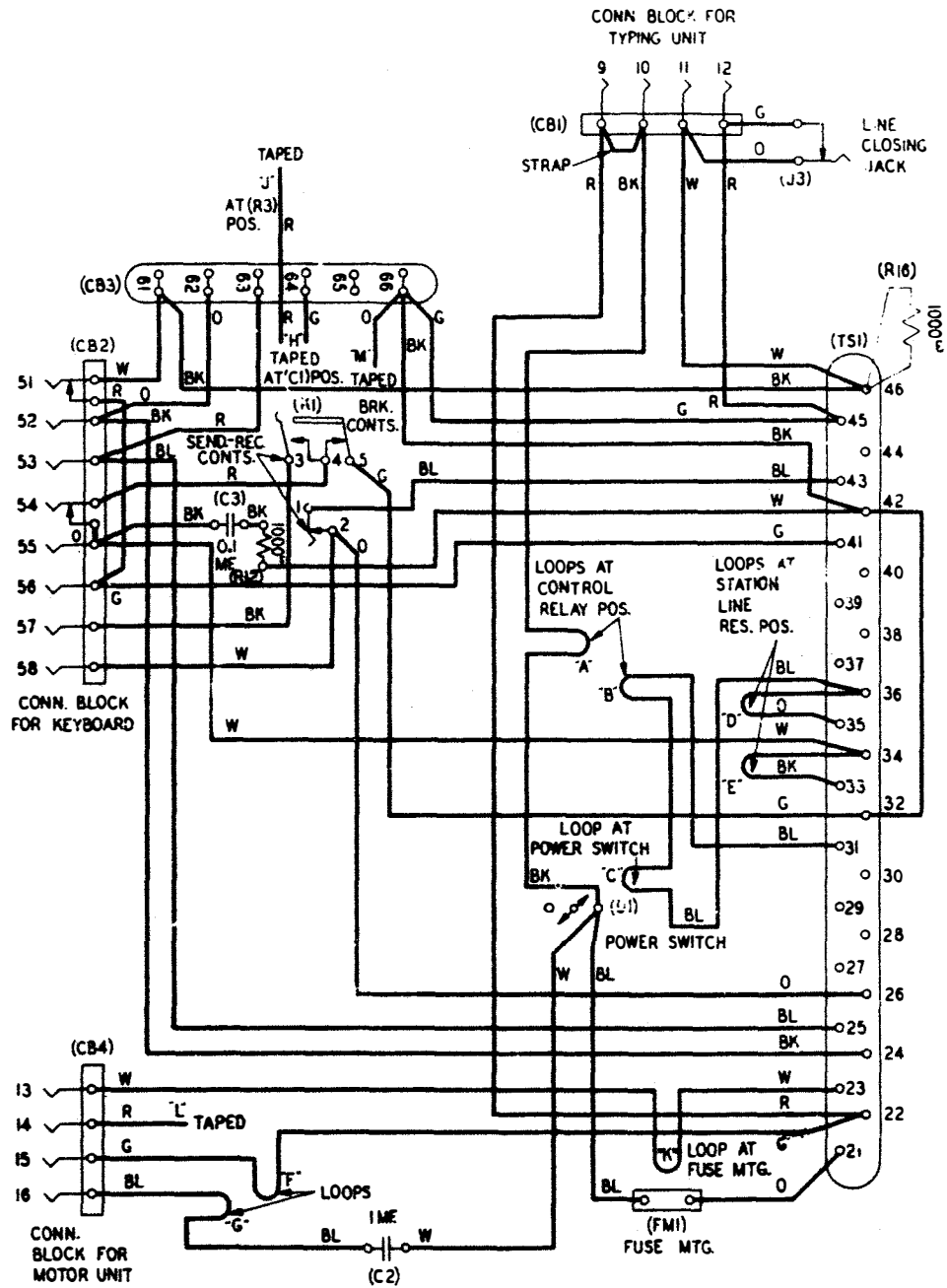
Figure 3 - 15C Teletypewriter Base
