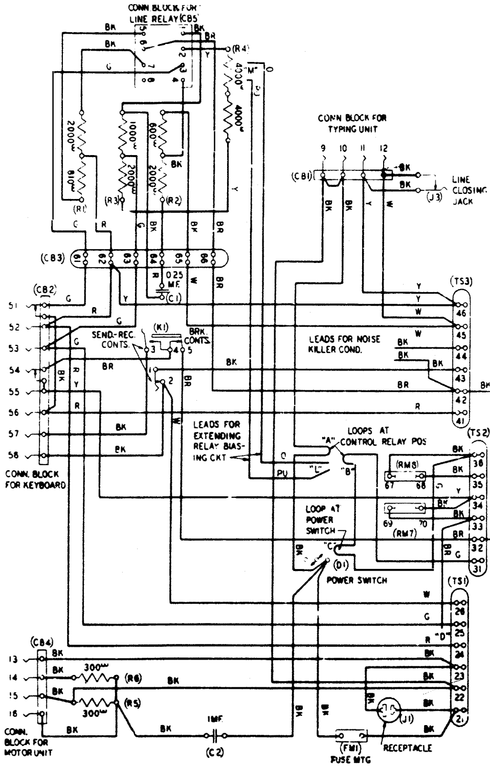
Figure 2 - 15B Teletypewriter Base
