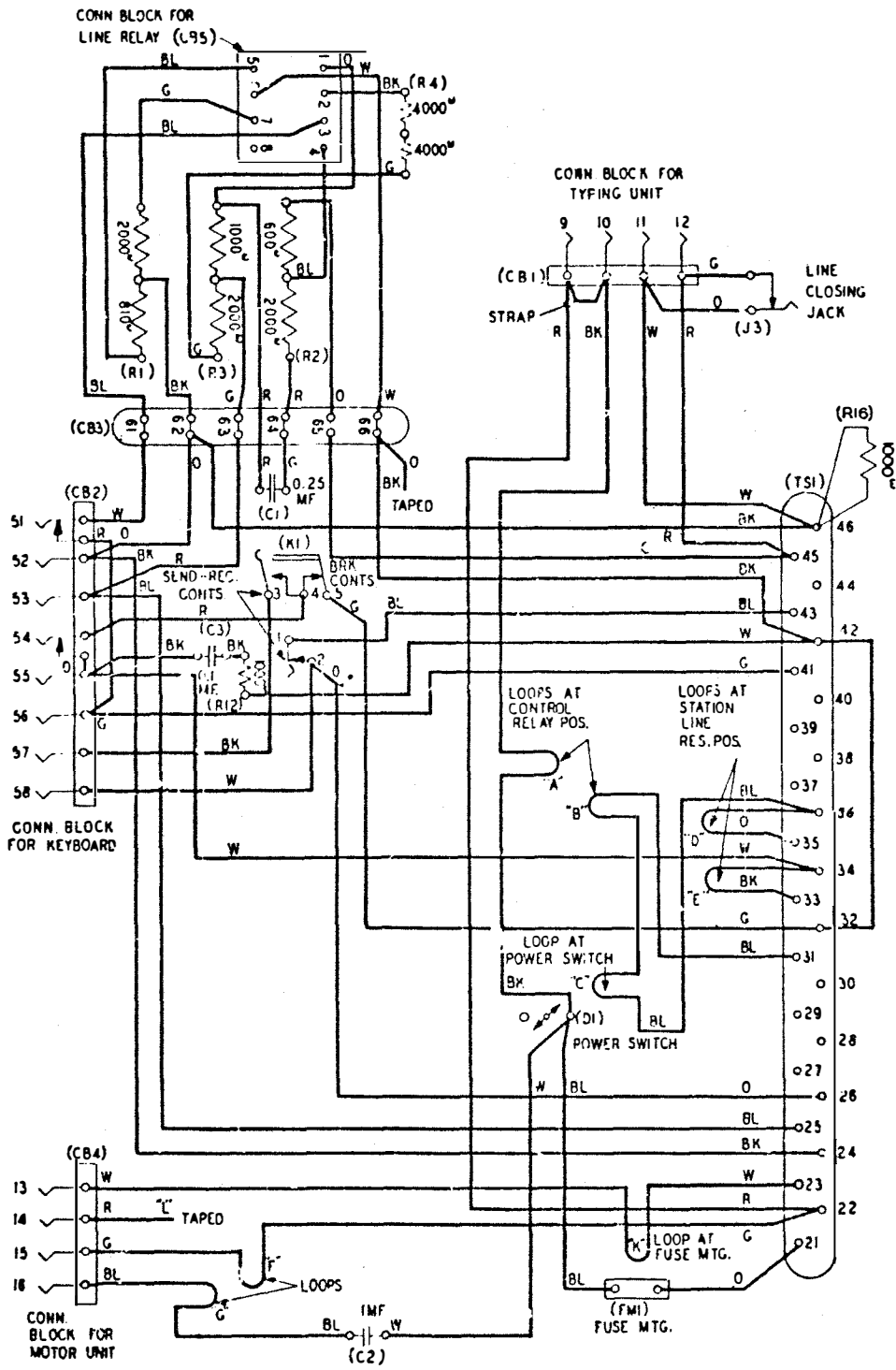
Figure 4 - 15D Teletypewriter Base
