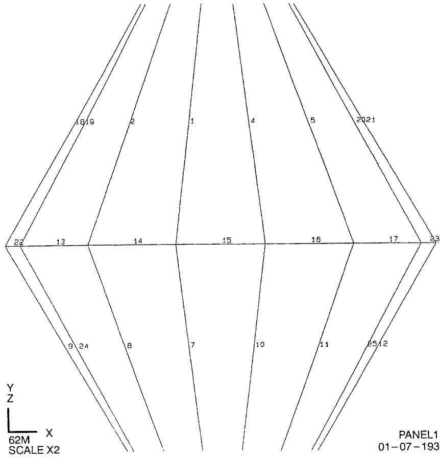
Figure 3. CFG2 panel.
