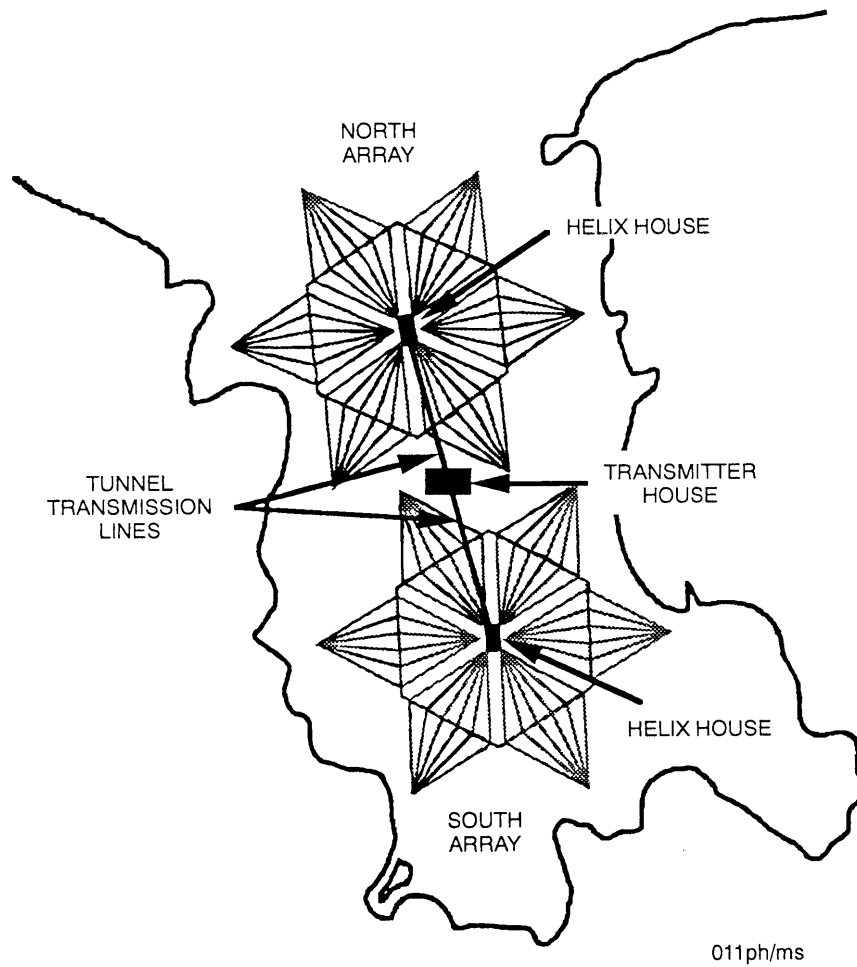
Figure 1. VLF Cutler.
